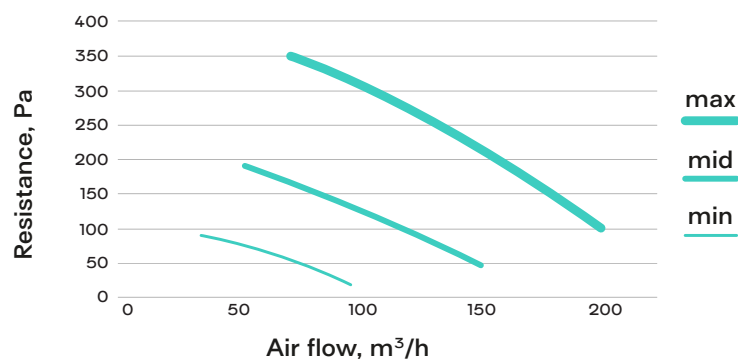
Performance curves
